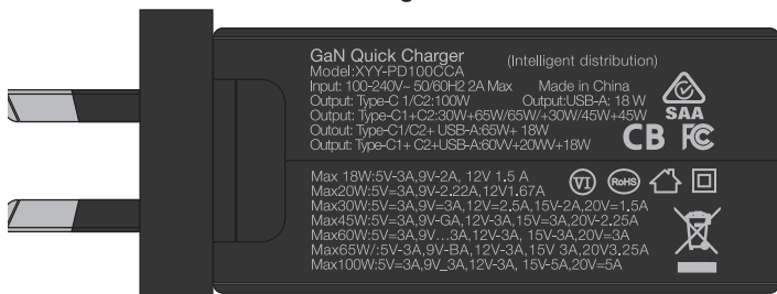
Top Side (When Plugged in)
