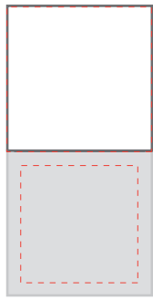
Front Top Mould Max. Area 21 x 21 mm
